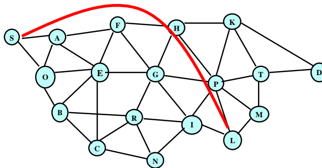
Fig.2 Wormhole Attack
